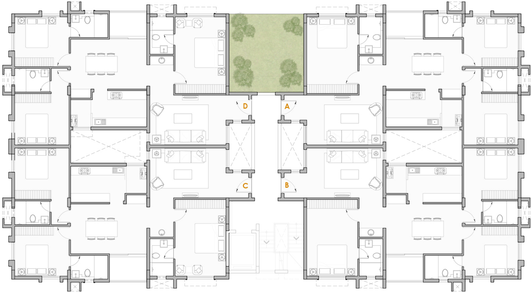
TYPICAL FLOOR
